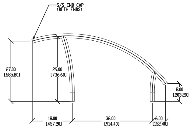
Deck-Mounted Hand Rail 1005
